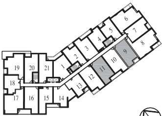
2ND TO 6TH FLOOR PLAN
